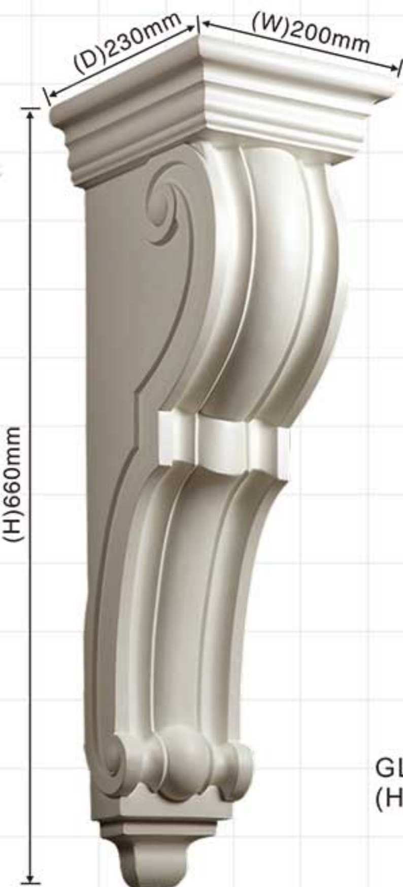
GL-6041 (H)660x(W)200x(D)230mm
