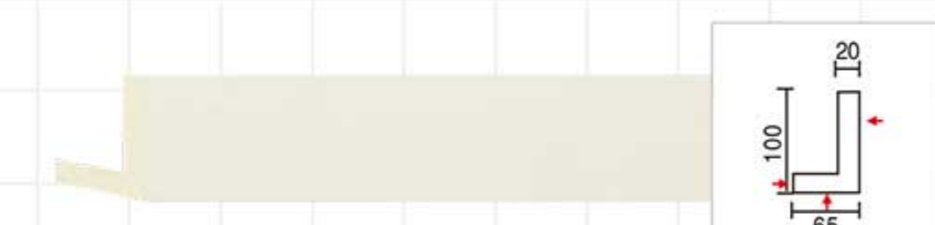
GD-82095-65 L:2400mm
