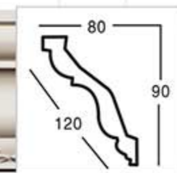
GA-81056 L:2400mm Breadth:120mm Pattern:60mm
