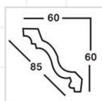
GC-83038-60 Length □ 2400mm Breadth: 85mm
