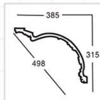
GA-81170 L:2400mm Breadth:498mm Pattern:244mm
