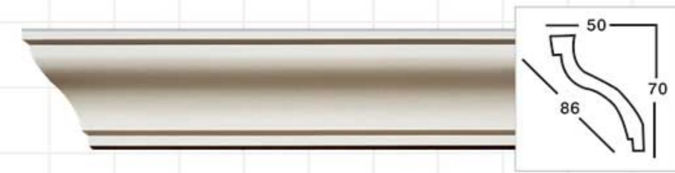
GC-83027-70 L:2400mm Breadth:86mm
