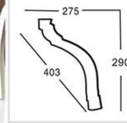
GA-81171 L:2100mm Breadth:403mm Pattern:60mm
