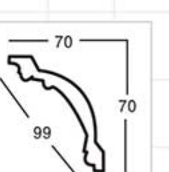
GA-81060-70 L:2400mm Breadth:99mm Pattern:100mm
