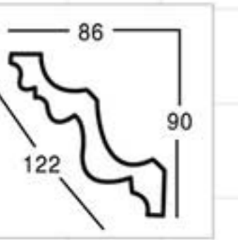
GA-81057 L:2400mm Breadth:122mm Pattern:122mm
