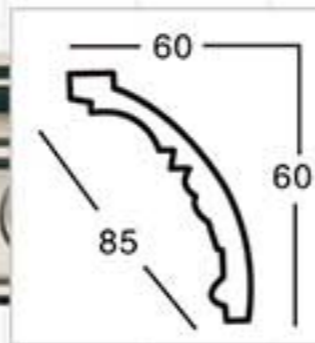
GA-81051-60 L:2400mm Breadth:85mm Pattern:180mm
