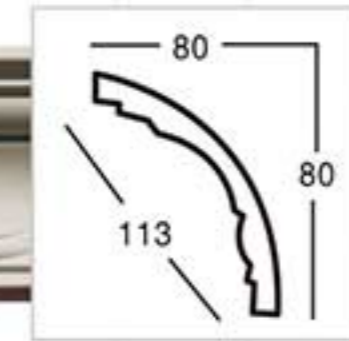
GA-81055 L:2400mm Breadth:113mm Pattern:200mm
