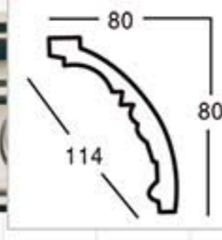
GA-81051-80 L:2400mm Breadth:114mm Pattern:200mm
