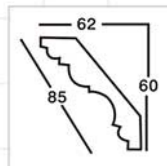
GC-83022-80 Length □ 2400mm Breadth: 85mm
