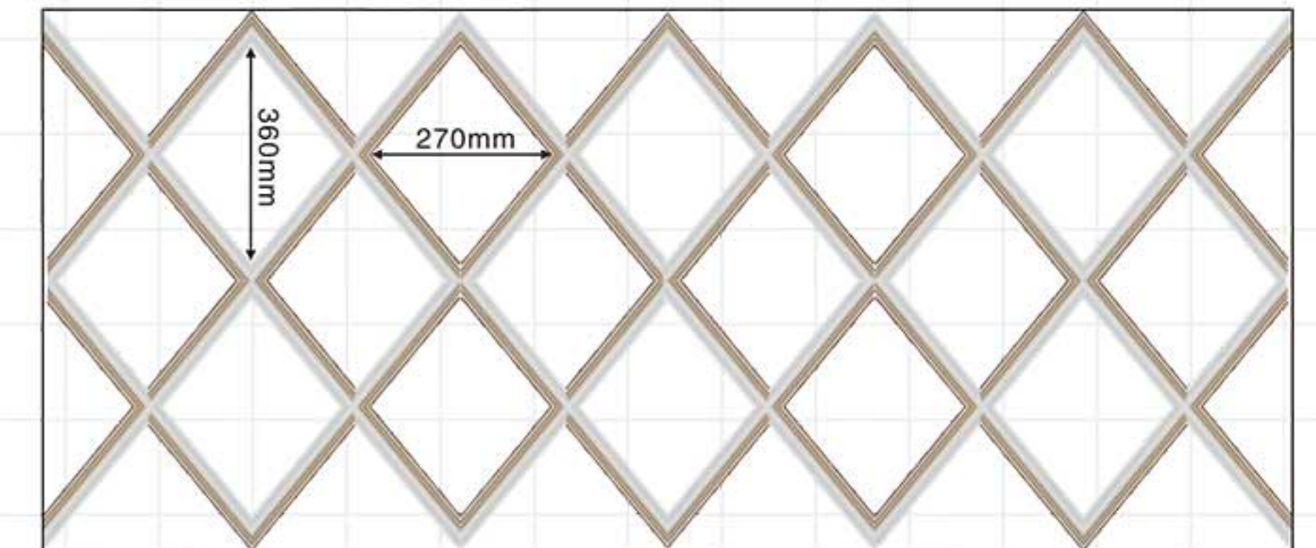
M-7409 D:460x300x15mm
