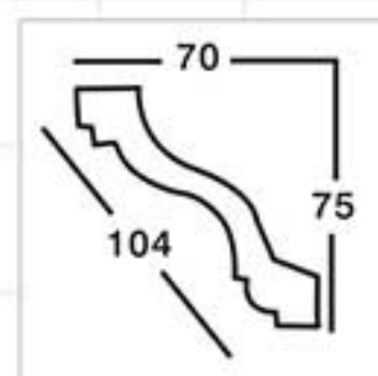
GC-83031-75 Length □ 2400mm Breadth: 104mm
