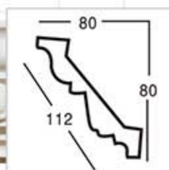
GA-81046 L:2400mm Breadth:112mm Pattern:32mm
