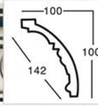
GA-81051-100 L:2400mm Breadth:142mm Pattern:220mm
