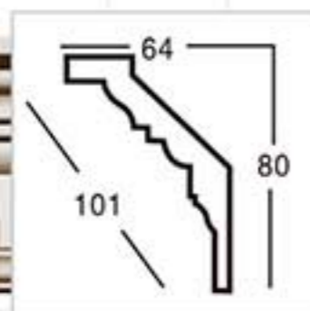
GA-81045 L:2400mm Breadth:101mm Pattern:45mm
