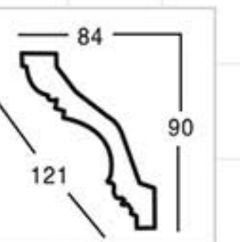
GA-81058 L:2400mm Breadth:121mm Pattern:40mm
