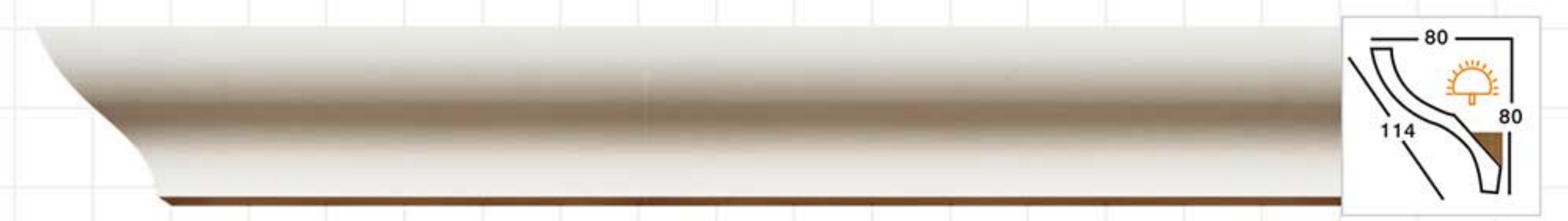
GC-83056-80 L:2400mm Breadth:114mm
