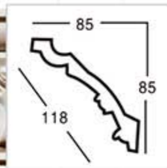
GA-81044-85 L:2400mm Breadth:118mm Pattern:150mm
