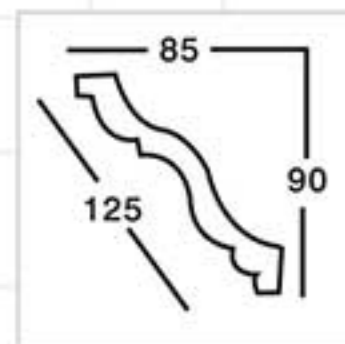
GC-83050 Length □ 2400mm Breadth: 125mm
