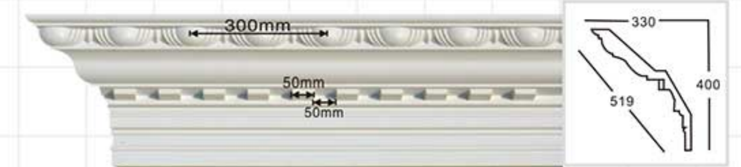
GA-81179 L:2100mm Breadth:519mm Pattern:300mm
