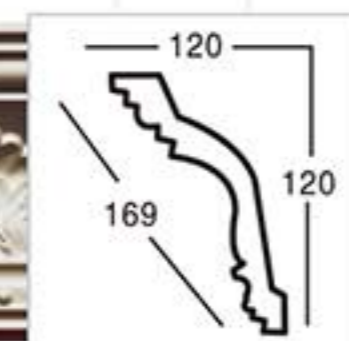
GA-81052-120 L:2400mm Breadth:169mm Pattern:86mm
