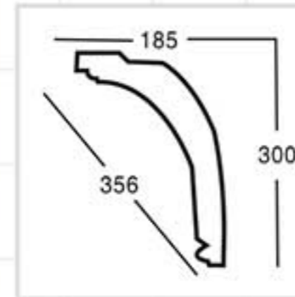
GA-81169 L:2400mm Breadth:356mm Pattern:122mm
