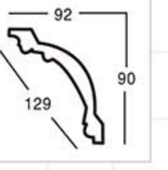
GA-81060-90 L:2400mm Breadth:129mm Pattern:100mm
