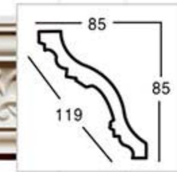
GA-81053 L:2400mm Breadth:119mm Pattern:101mm
