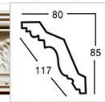
GA-81052-85 L:2400mm Breadth:117mm Pattern:49mm
