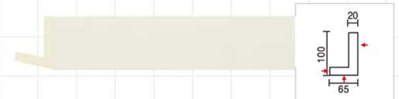
GD-85095-65 L:2400mm
