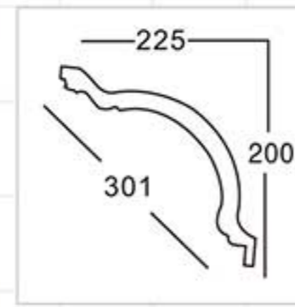
GA-81167 L:2400mm Breadth:301mm Pattern:100mm
