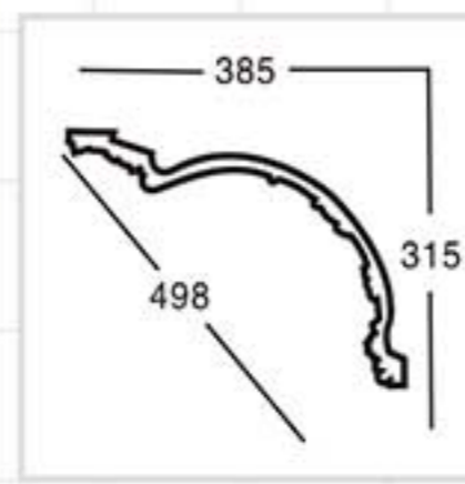
GA-81170 L:2400mm Breadth:498mm Pattern:244mm
