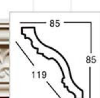
GA-81053 L:2400mm Breadth:119mm Pattern:101mm
