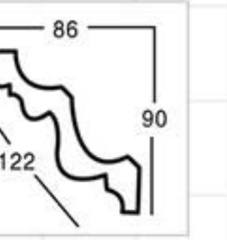
GA-81057 L:2400mm Breadth:122mm Pattern:122mm
